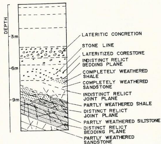
Fig. 1 Schematic diagram of the main features of the morphological horizons of the Kenny Hill Formation from Raj (1983)
