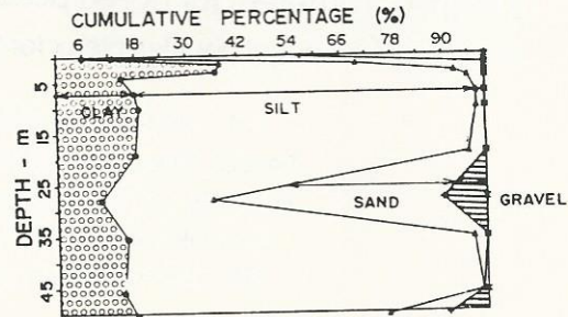
Fig. 4 Grain Size Distribution at a typical site
