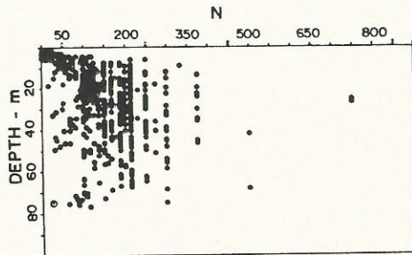
Fig. 2 N values at a typical site.
