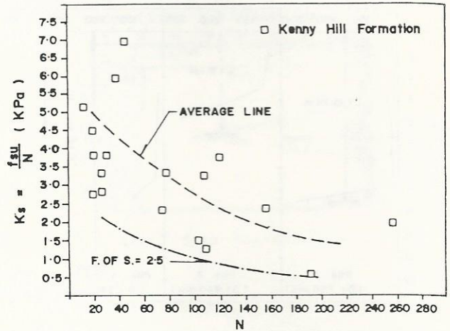
Fig. 7 Shaft Resistance Factor, K_s , versus N
