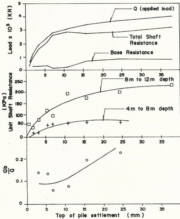
Fig. 6 Applied Load, Base Load, Shaft Resistance versus settlement - Pile 9
