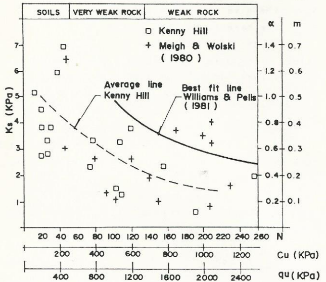
Fig. 8 Comparison of Shaft Resistance Factors
