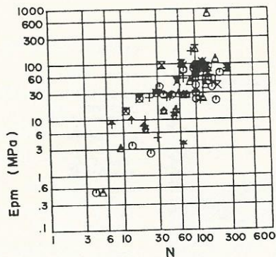
Fig. 3 Pressuremeter Modulus versus N for the Kenny Hill Formation from Toh et al. (1987)
