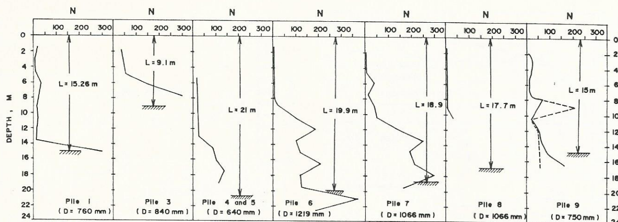
Fig. 5 Profiles of N and Pile Dimensions
