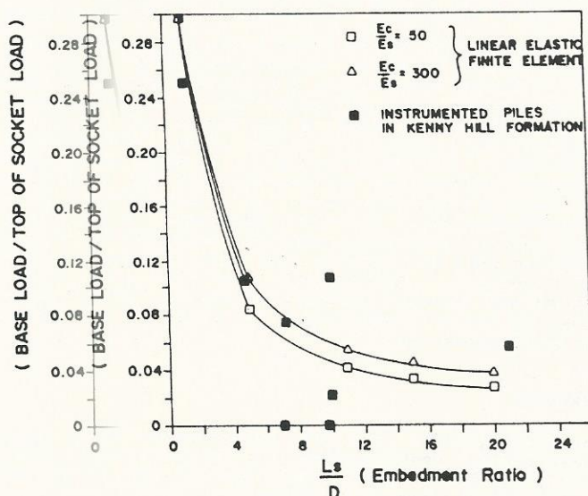
Fig. 10 Proportion of Base Load as a Function of Embedment Ratio
