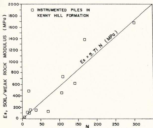
Fig. 9 Soil/Weak Rock Modulus versus N
